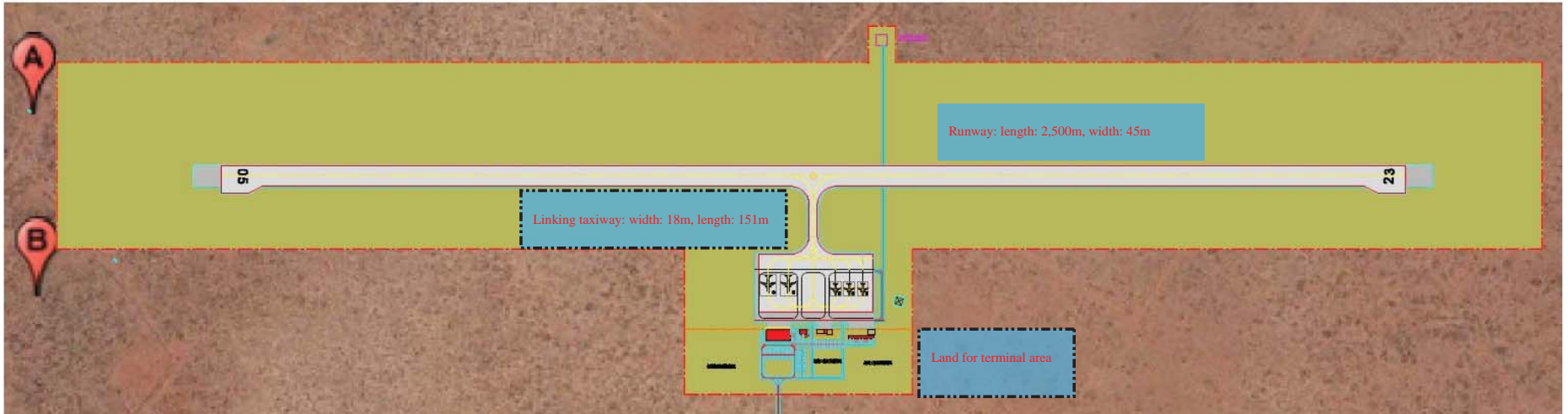
Fig. 4-4 General Layout Plan of Terminal Area
